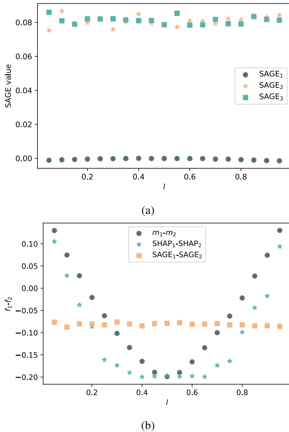
FIGURE 3. The (a) SAGE values for the DGP in (4) across a grid of 0.05 \leq \ell \leq 0.95 , (b) Shapley values for the mean absolute SHAP, SAGE and m function formulations, for the difference \varphi_1 - \varphi_2 between attribution to X_1 and X_2 , across the same range of \ell values. Similar results were observed for the difference \varphi_1 - \varphi_3 . Values \varphi_1 - \varphi_2 < 0 indicate regions of the parameter space for which model selection results are inadequate.
