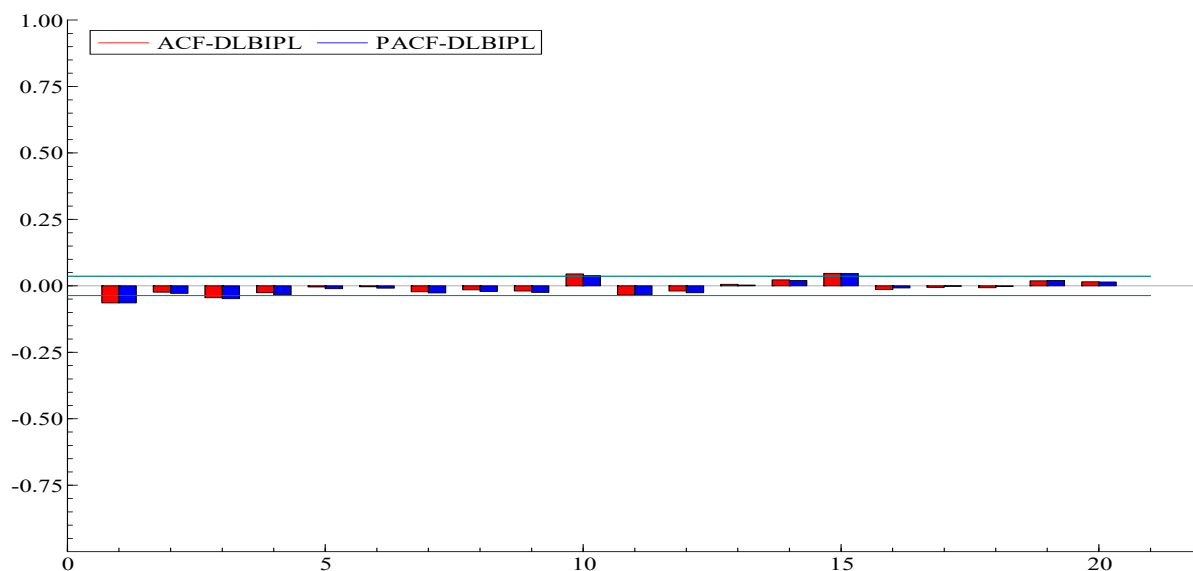
Figure 3. The ACF and PACF of BIPL.
