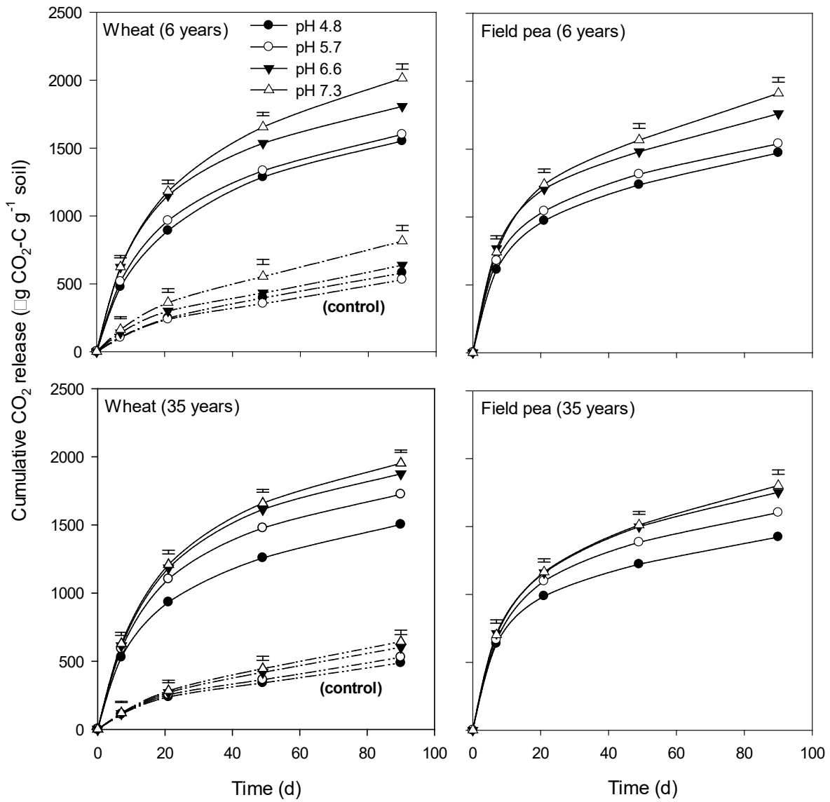
Figure 1. Cumulative total CO 2 release from soils incubated without residue (control) or with wheat (left) or field-pea (right) residue. The soils differing in initial pH were from two lime trials with either 6 (top) or 35 years (bottom) since liming. Vertical bars indicate the least significant difference ( P=0.05 ) between means for each sampling time.
