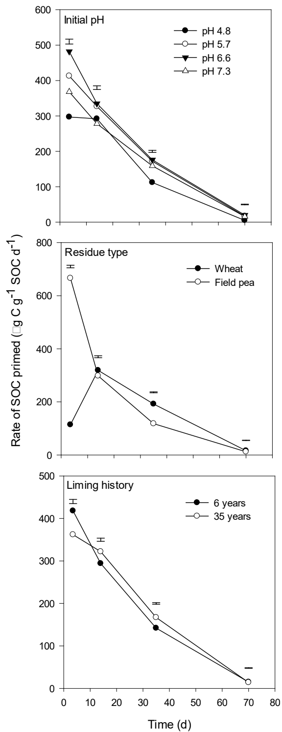
Figure 3. The main effects of initial pH, residue type and liming history on the rate of soil organic C mineralization (SOC primed), in response to the addition of wheat or field-pea residue to soils differing in initial pH. The soils were from lime trials with either 6 or 35 years since liming. Vertical bars indicate the least significant difference ( P=0.05 ) between means for each sampling time.
