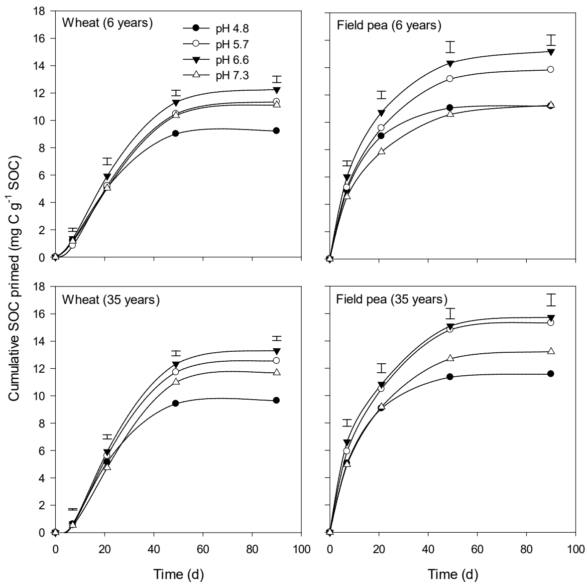
Figure 2. Cumulative amount of primed C per gram of indigenous SOC over 90 days in response to the addition of wheat (left) or field-pea (right) residue to soils differing in initial pH. The soils were from two lime trials with either 6 (top) or 35 years (bottom) since liming. Vertical bars indicate the least significant difference ( P=0.05 ) between means for each sampling time.
