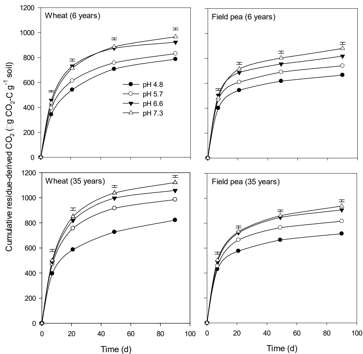
Figure 4. Cumulative residue-derived CO 2 release of soils differing in initial pH incubated with wheat (left) or field-pea (right) residue. The soils were from two lime trials with either 6 (top) or 35 years (bottom) since liming. Vertical bars indicate the least significant difference ( P=0.05 ) between means for each sampling time.
