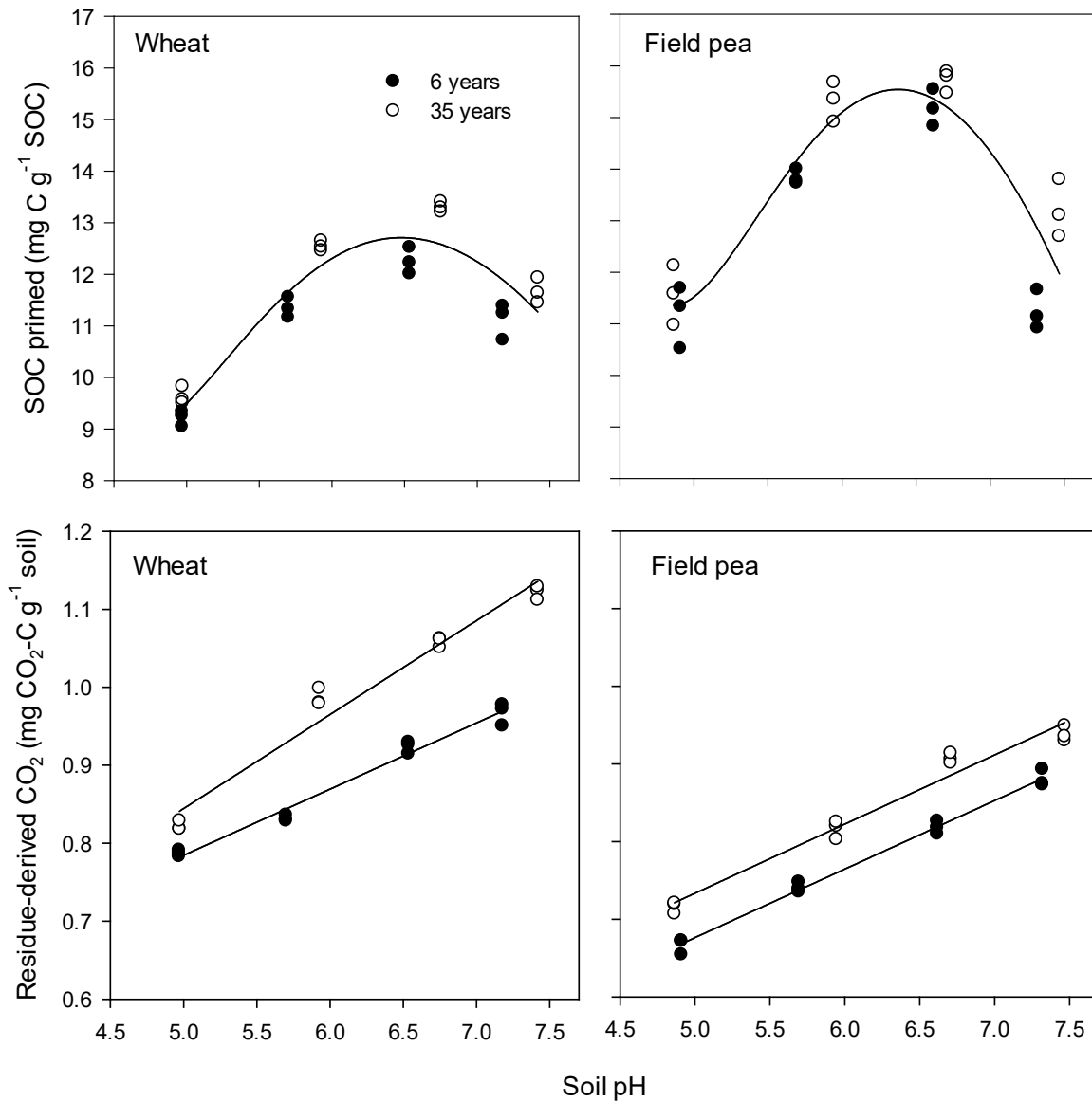
Figure 6. Relationships between initial soil pH and the amounts of soil organic C (SOC) primed in response to the addition of wheat or field-pea residue to soils from two lime trials with either 6 or 35 years since liming (top) and residue decomposed (bottom).
