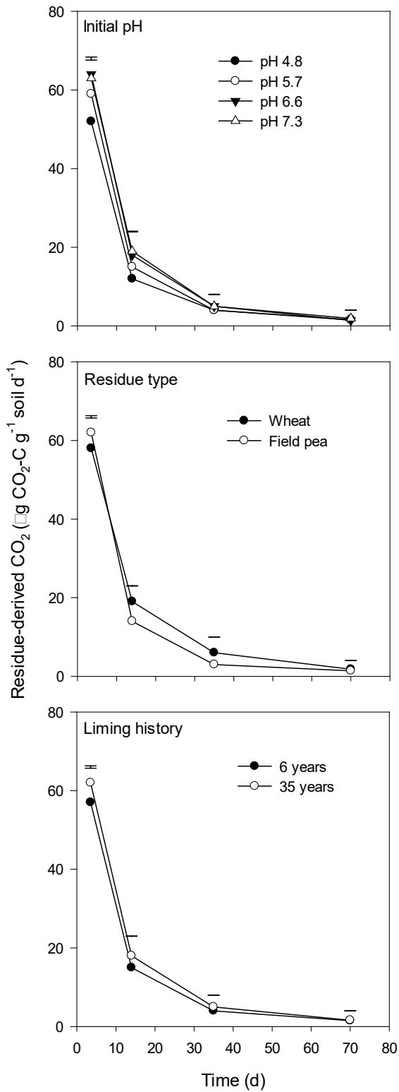
Figure 5. The main effects of initial pH, residue type and liming history on the rate of residue-derived CO 2 release in response to the addition of wheat or field-pea residue to soils differing in initial pH. The soils were from two lime trials with either 6 or 35 years since liming. Vertical bars indicate the least significant difference ( P=0.05 ) between means for each sampling time.
