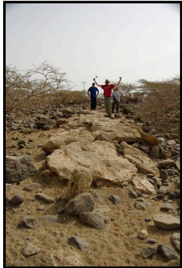
Figure 13: Outcrop of coral/wadi calcrete at WP 275 at 40m asl and 3 km from coast.
