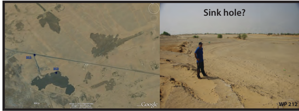
Figure 12: Google Earth image (l) showing kilometre-wide depressions a few kilometres from the modern coastline, potential sinkholes, and (r) the appearance of the southernmost depression from WP212.
