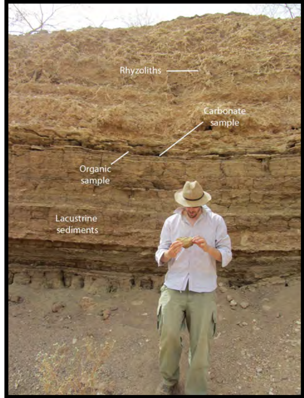
Figure 19: Lacustrine sediments showing location of samples. Note major distinction between laminated lacustrine sediments at base of section and terrestrial sediments at dominated by rhizoliths at the top of the section.
