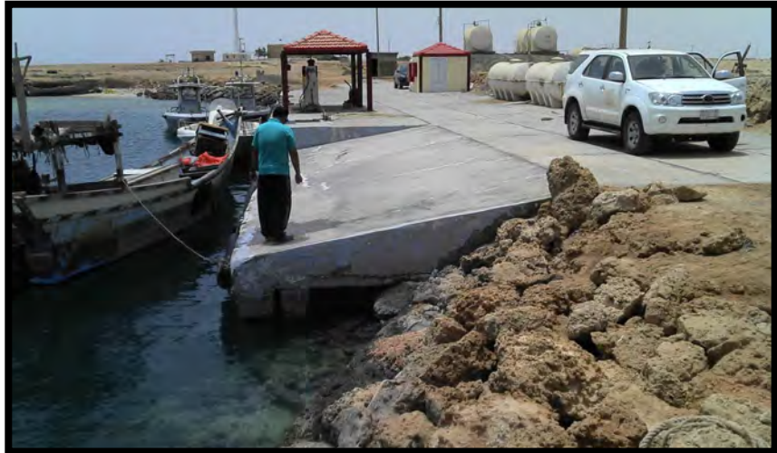
Figure 22: The temperature loggers are located at the foot of the quayside in protected waters, sheltered from both rough weather and fishing boats.
