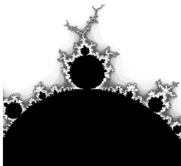
Figure 3. Mandelbrot Set.
