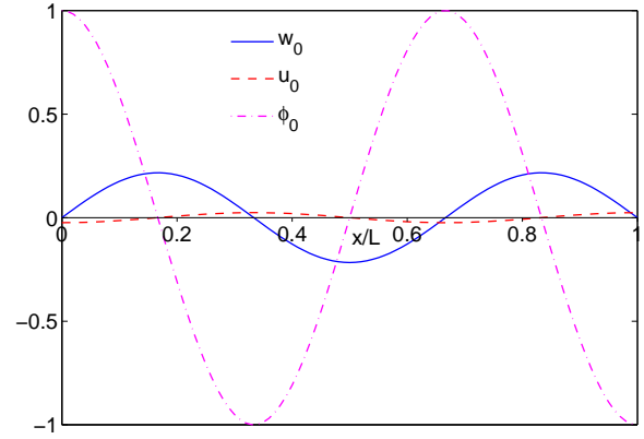
(f) Mode 3, \bar{\omega}_3=47.5396 ( 0^\circ/90^\circ )
