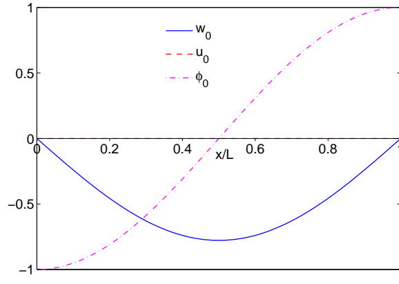
(a) Mode 1, \bar{\omega}_1=13.6136 ( 0^\circ/90^\circ/0^\circ )
